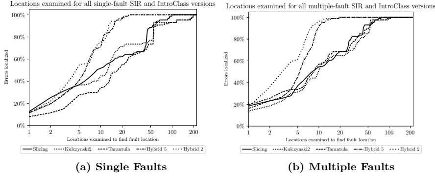
Fig. 11 Cumulative frequency of the locations to be examined for (a) single-fault and (b) multiple-fault versions of the SIR and IntroClass , using the hybrid approach, statistical debugging ( Kulczynski2 and Tarantula ) and dynamic slicing
